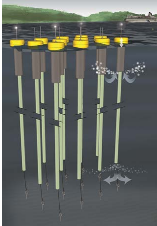
Figure 3.14. Concept of a possible full-scale application and design of CoreOceanPump.
