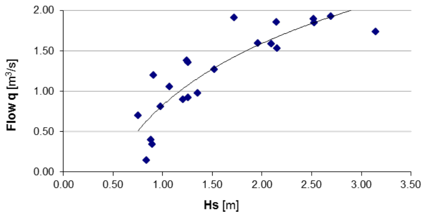
Figure 3.6. Calculated average flows in the WEBAP I pilot as a function of significant wave height H_s .
