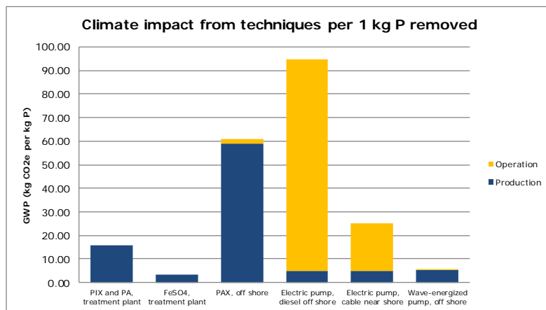
Figure 3.10. Climate impact from the different techniques.
