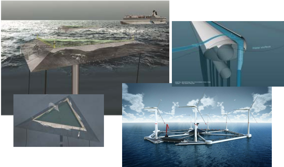
Figure 3.12. Concept of a possible full-scale application and design of WEBAP I as an independent unit or in combination with other offshore structures (here Hexicon offshore wind; www.hexicon.eu ).
