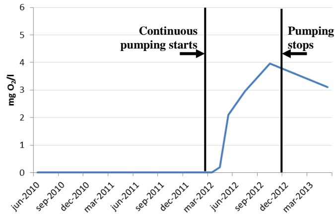
Figure 3.7. Oxygen concentration (mg/l) June 2010-May 2013 in the bottom water in Kanholmsfjärden adjacent to the WEBAP II pilot.
