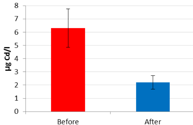
Figure 3.9. Cadmium concentrations in Kanholmsfjärden surface and deep water before (n = 4) and after (n = 2) oxygenation.
