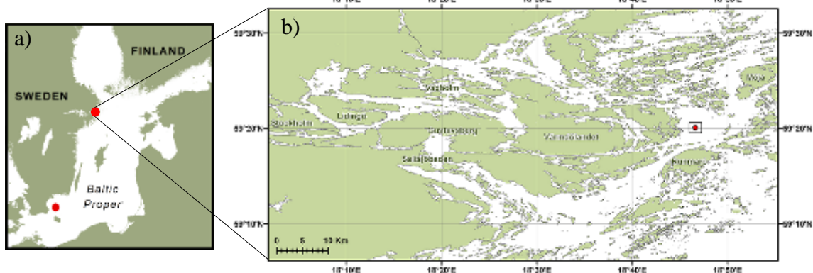
Figure 3.3. Map of the Baltic Sea with the study area Hanöbukten and the study area Kanholmsfjärden in the Stockholm archipelago.
