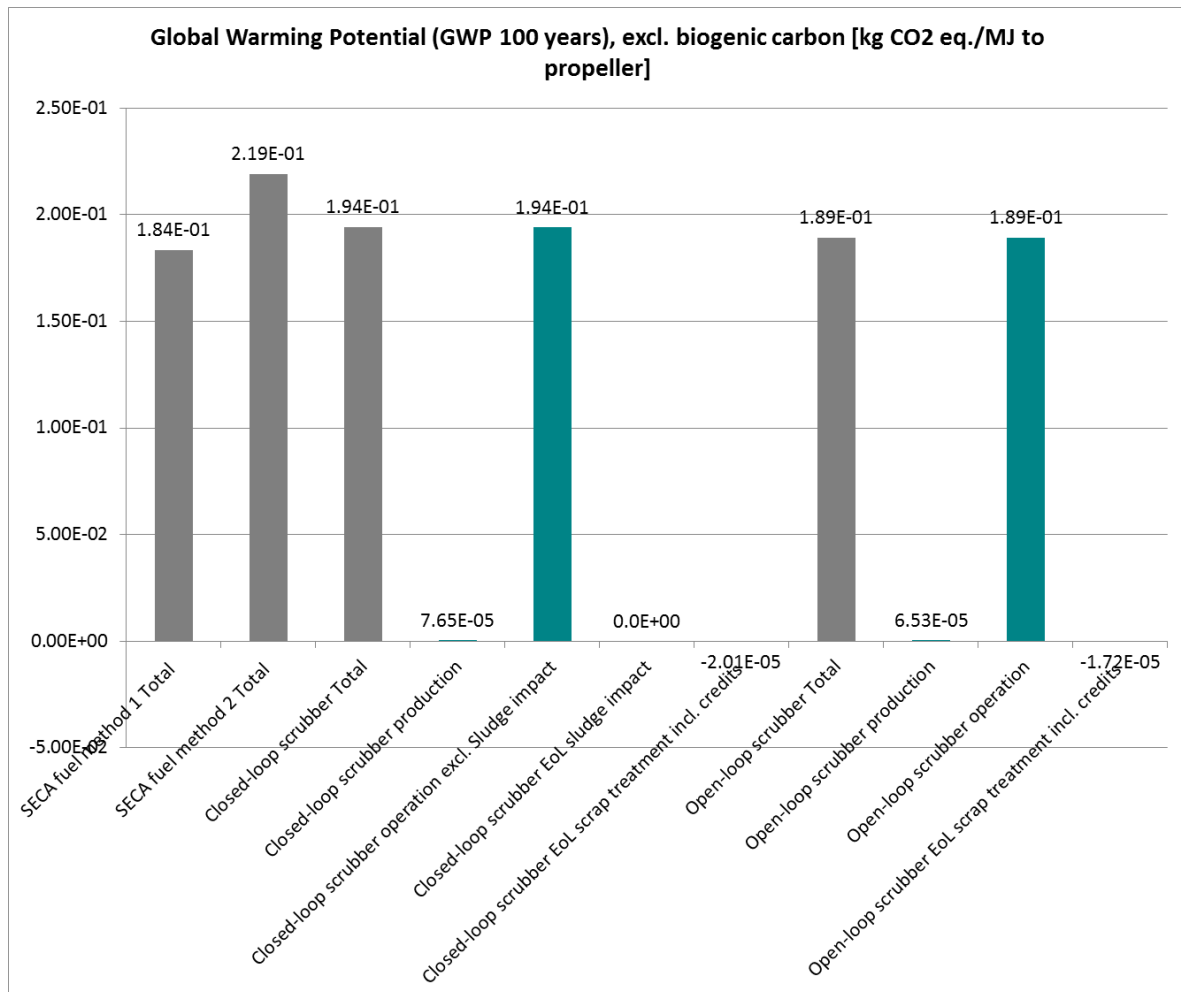
Figure B Comparison of Global Warming Potential (GWP 100) between the three different cases in the study (SECA fuel, Closed-loop scrubber, and Open-loop scrubber). For the SECA fuel, two different methods are shown. For the scrubber cases, the total impact as well as the different contributing shares (production, operation, and end-of-life) are shown. Negative values come from avoided processes in end-of-life. Grey bars show totals.
