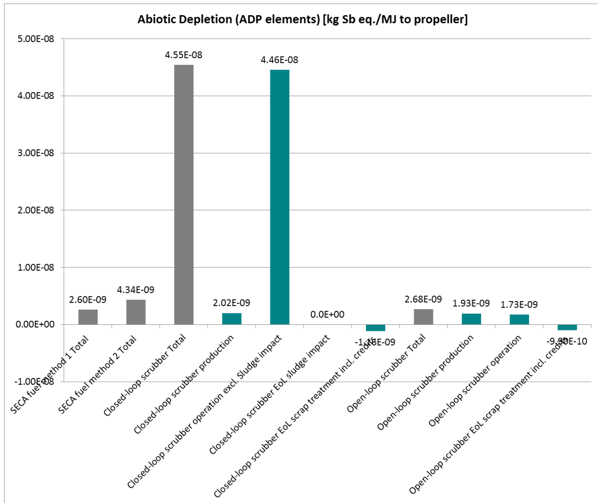
Figure 8.1 Comparison of Abiotic Depletion Potential (ADP elements) between the three different cases in the study (SECA fuel, Closed-loop scrubber, and Open-loop scrubber). For the SECA fuel, two different methods are shown. For the scrubber cases, the total impact as well as the different contributing shares (production, operation, and end-of-life) are shown. Negative values come from avoided processes in end-of-life. Grey bars show totals.
