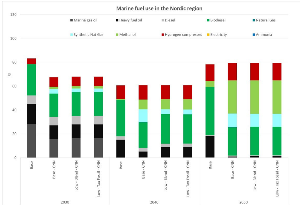
Figure 16. Fuel use in the future Nordic shipping sector (covering Denmark, Norway, and Sweden) for four different scenarios; Base scenario with moderate GHG emission reduction targets, Base carbon neutral Nordic (CNN) CNN with more stringent GHG reduction targets reaching carbon neutrality by 2050, Low Blend CNN with also blending mandate for renewable marine fuels and Low Tax Fossil CNN with CNN assumptions plus tax on fossil marine fuels.
